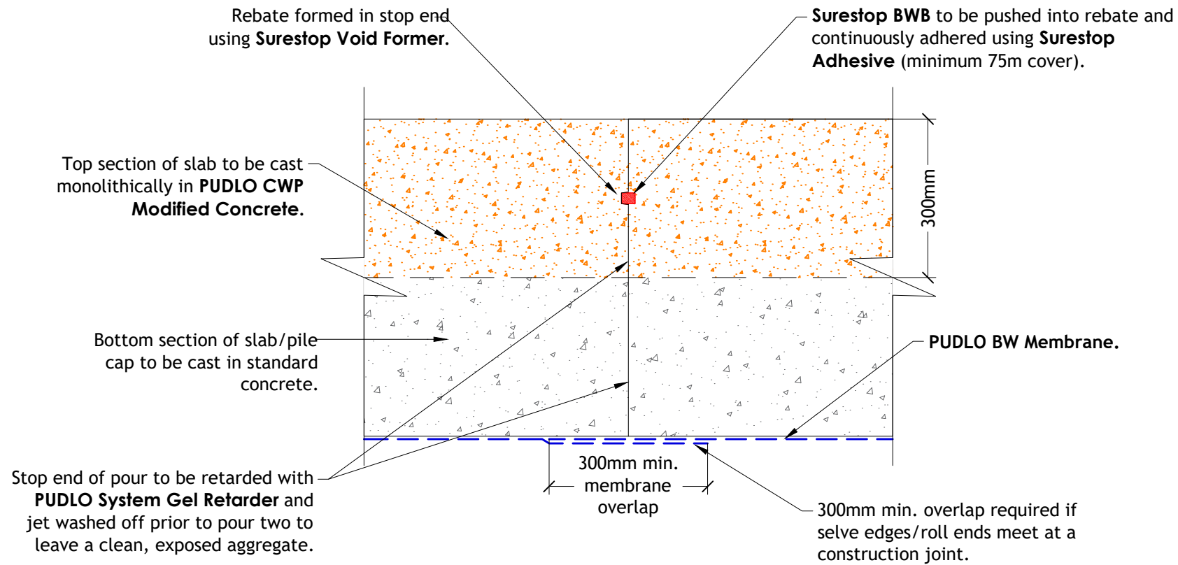
Alternative 1 Top & bottom sections of slab to be cast in the same pour
