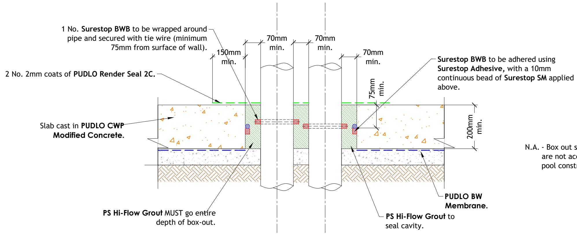
1 Box-out Penetration Detail Scale: 1:10
