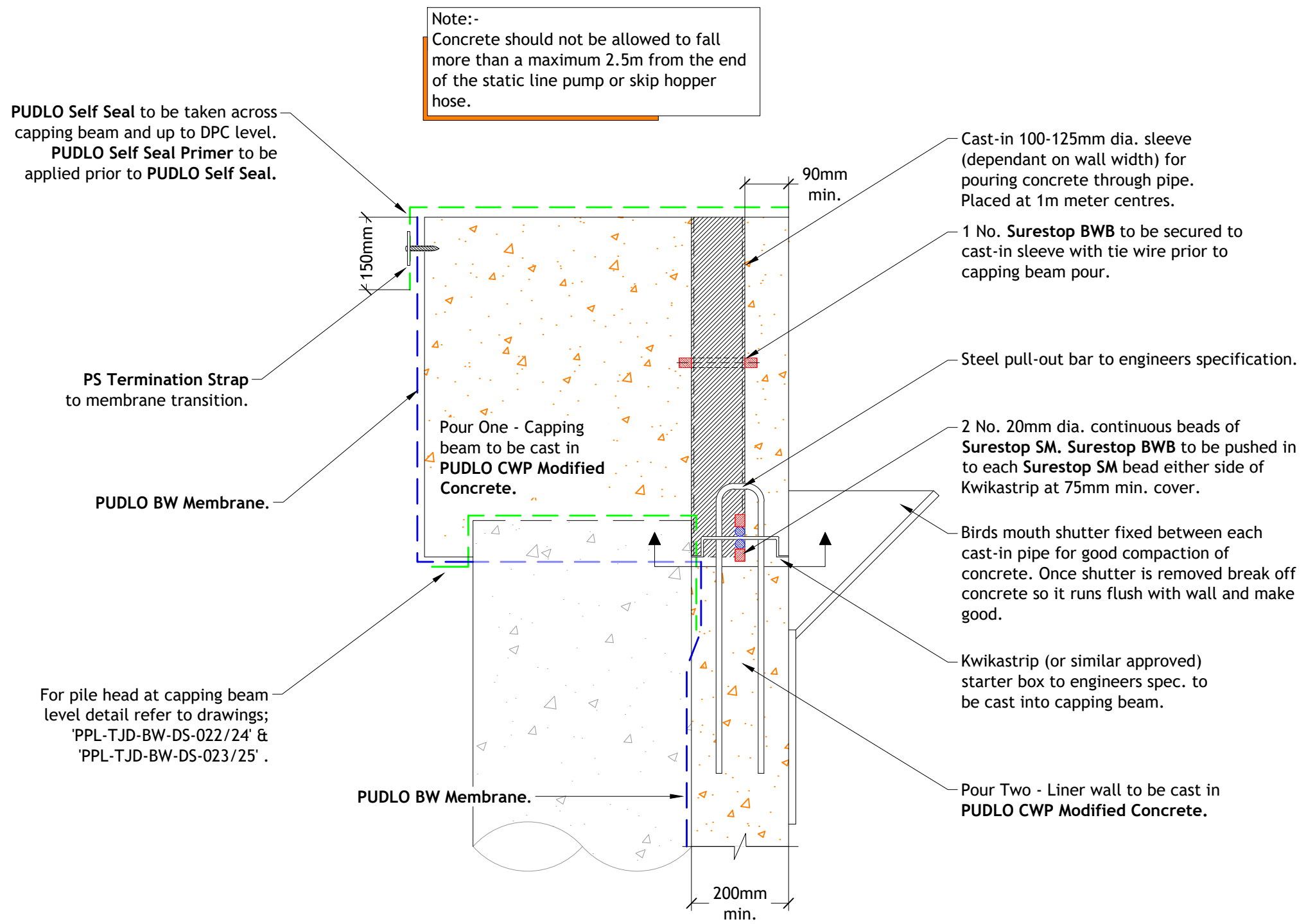
1 Capping Beam Detail Scale: 1:10
