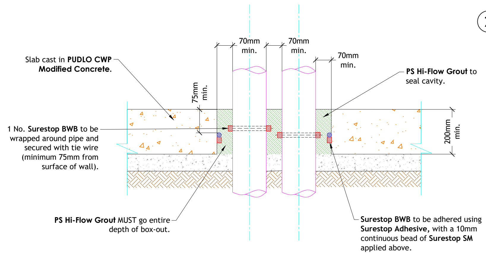
1 Box-out Penetration Detail Scale: 1:10
