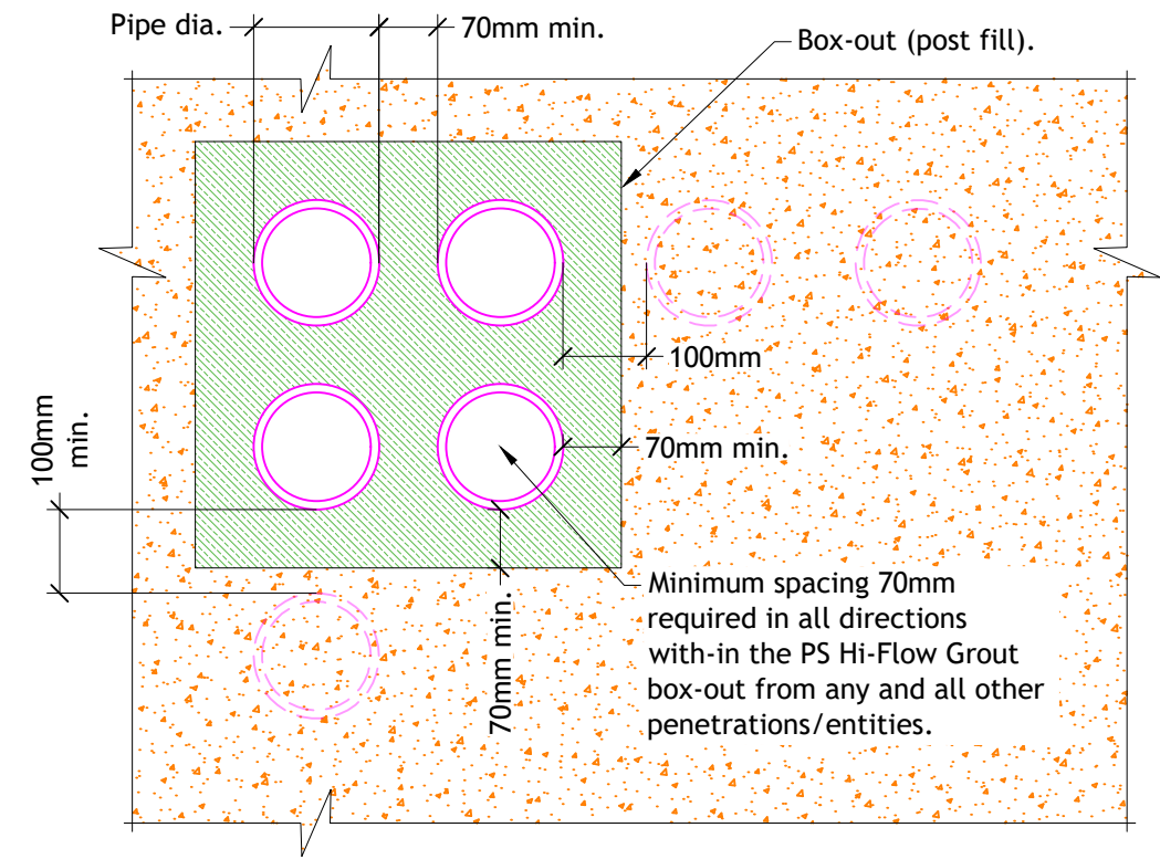
2 Penetration Spacing Detail Scale: 1:10
