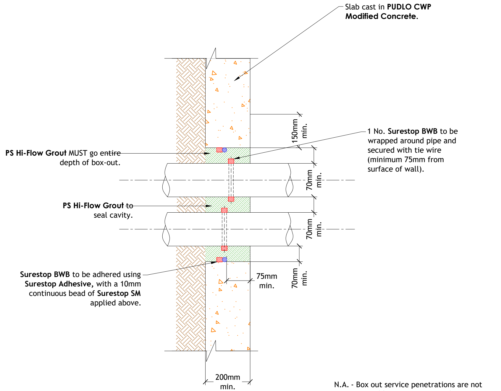
1 Box-out Penetration Detail Scale: 1:10
