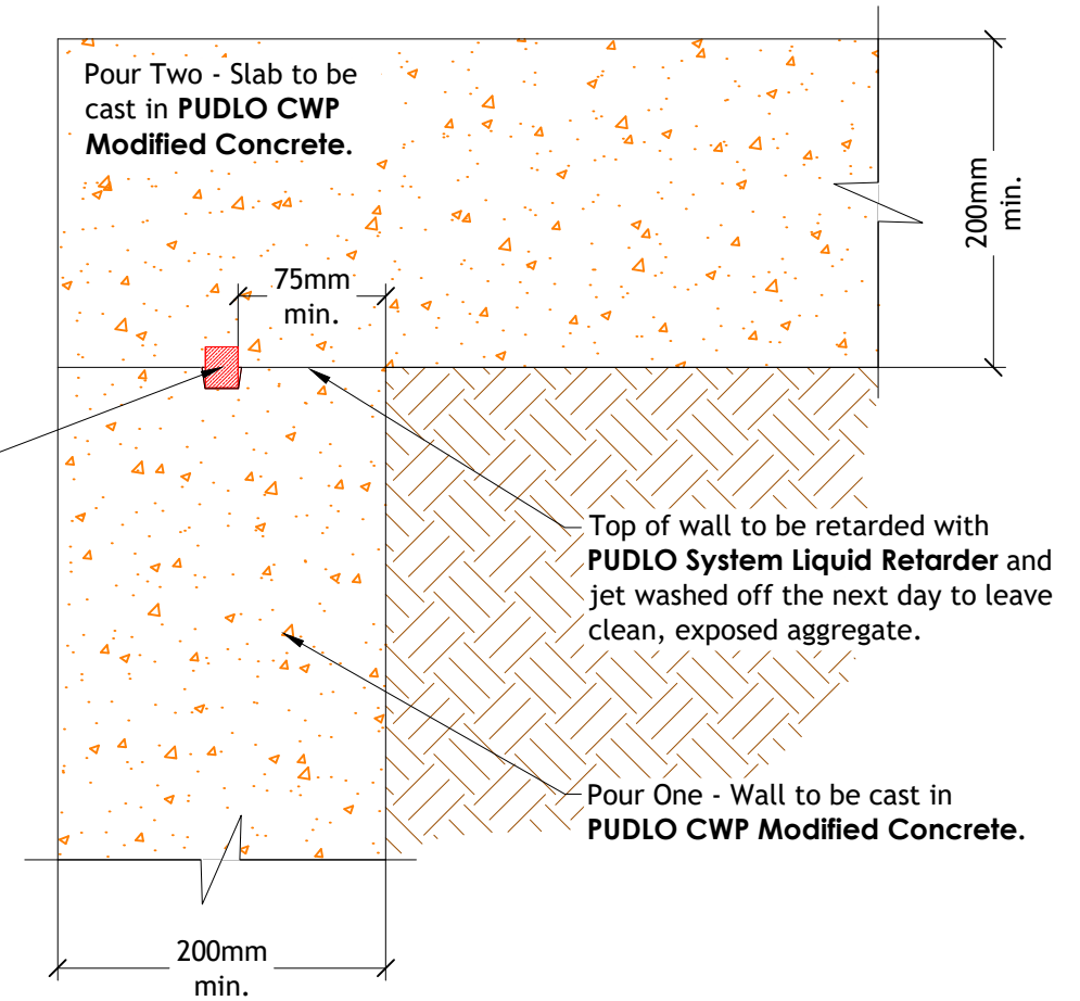
2 Wall Head at Ground Bearing Slab Scale: 1:5
