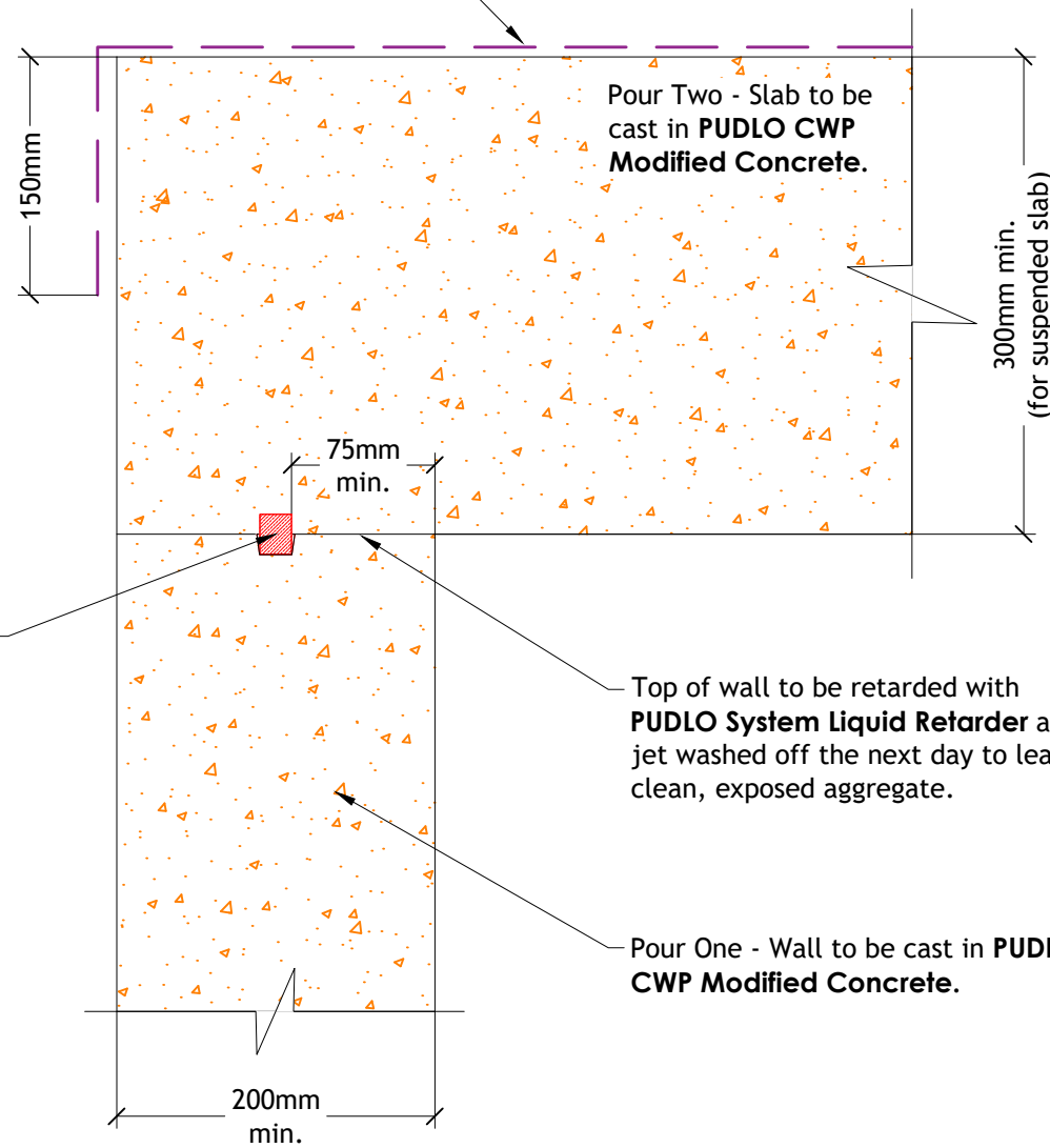
1 Wall Head at G/F Slab Scale: 1:5
