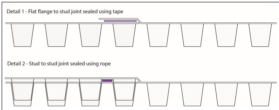
Figure 3 PUDLO CD Tape 28mm x 22m and PUDLO CD Rope 10 mm x 5 m sealing
