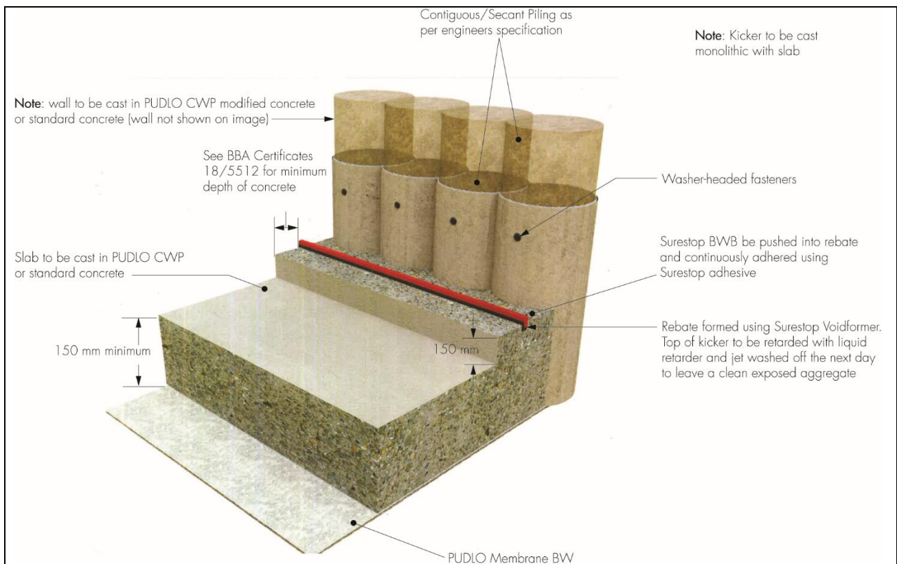
Figure 2 Surestop BWB installation details
