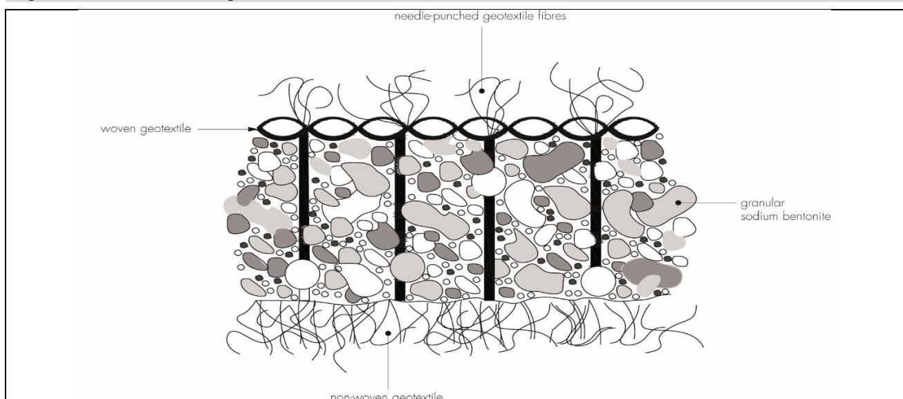
Figure 1 Cross-section through PUDLO Membrane BW
