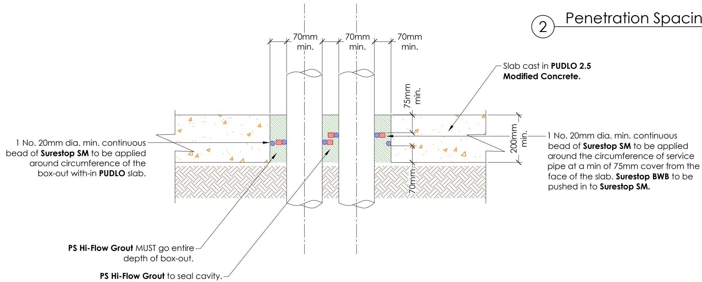
1 Box-out Penetration Detail Scale: 1:10
