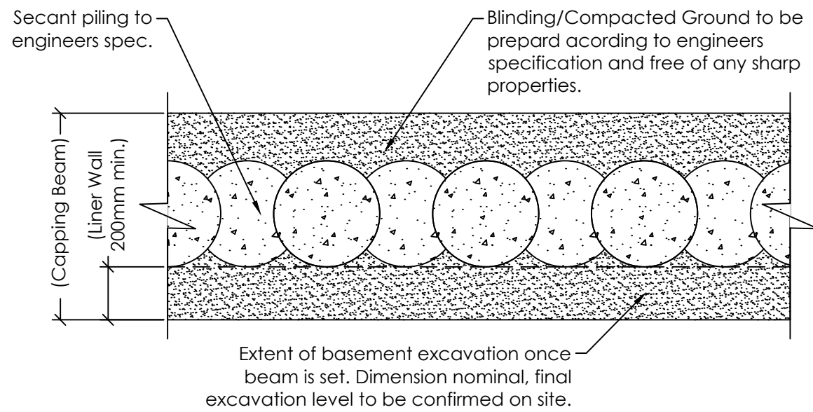
1 Secant Pile Head and Blinding Scale: 1:20
