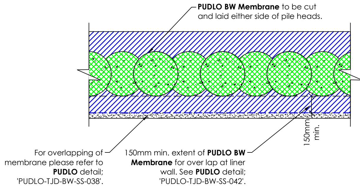
1 Secant Pile Head and Blinding Scale: 1:20
