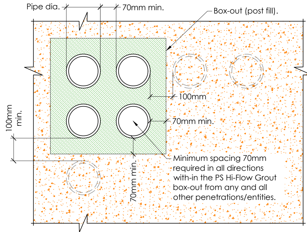
2 Penetration Spacing Detail Scale: 1:10
