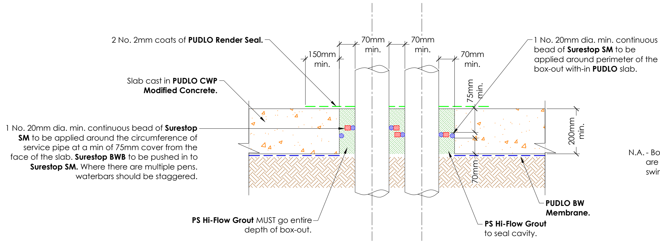
1 Box-out Penetration Detail Scale: 1:10
